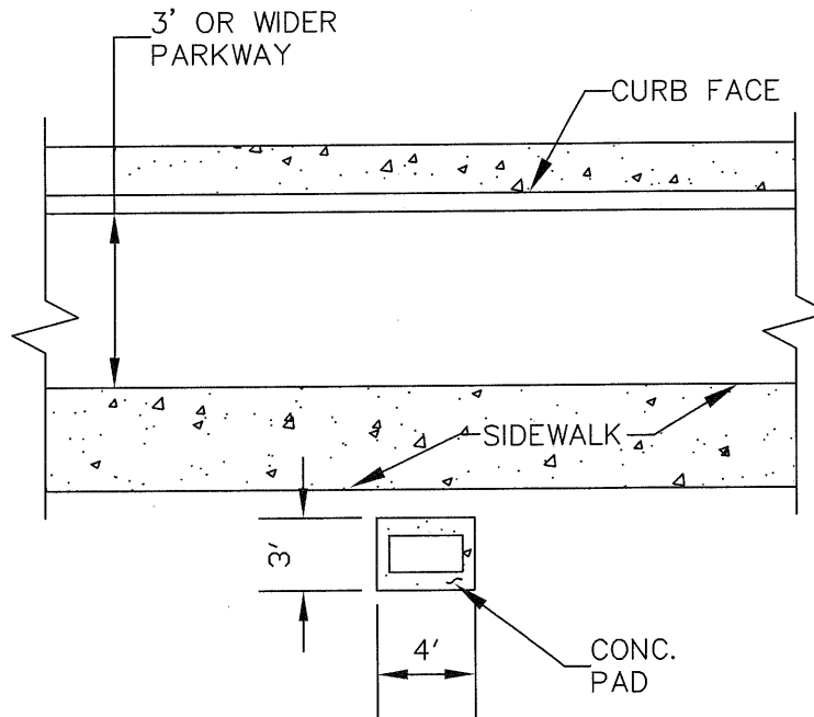
CASE II – SIDEWALK NOT ADJACENT TO CURB
