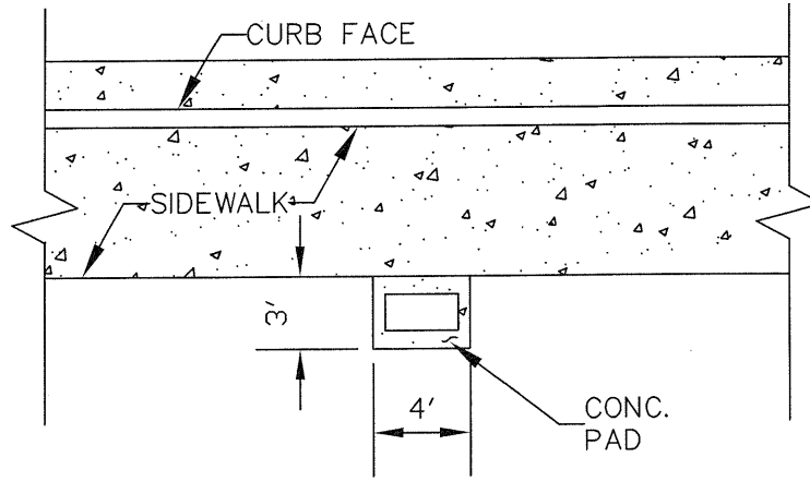
CASE I – SIDEWALK ADJACENT TO CURB
