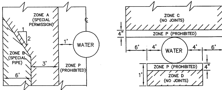
PARALLEL CONSTRUCTION
