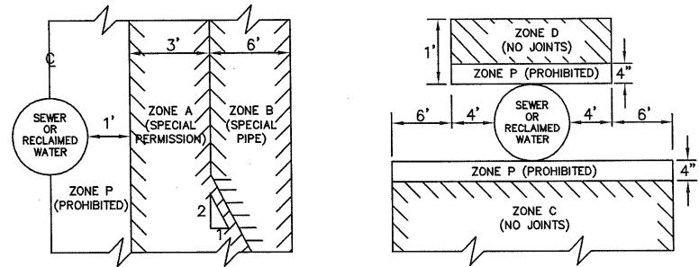
PARALLEL CONSTRUCTION
